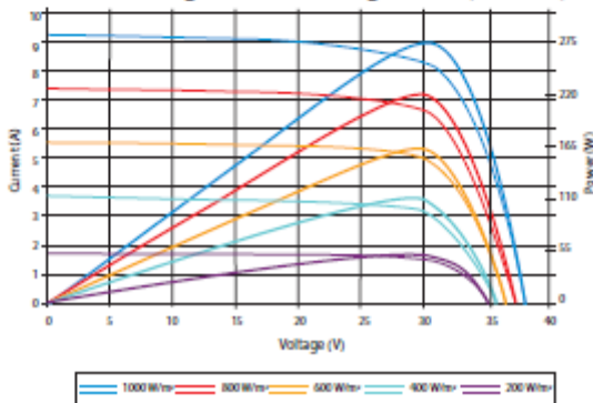
Current-Voltage & Power-Voltage Curve (275S-20)
